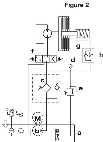
Figure 2: Hydraulic release, multidisc brake assembly in open circuit with hydraulic motor
